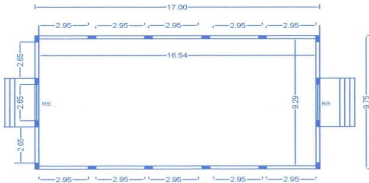
PLAN SCALE 1:100
