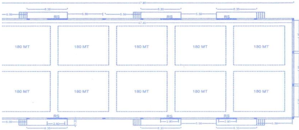
PLAN FOR 1800 MT WAREHOUSE SCALE 1:100
